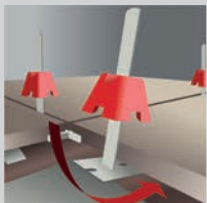
Position strap and cap
