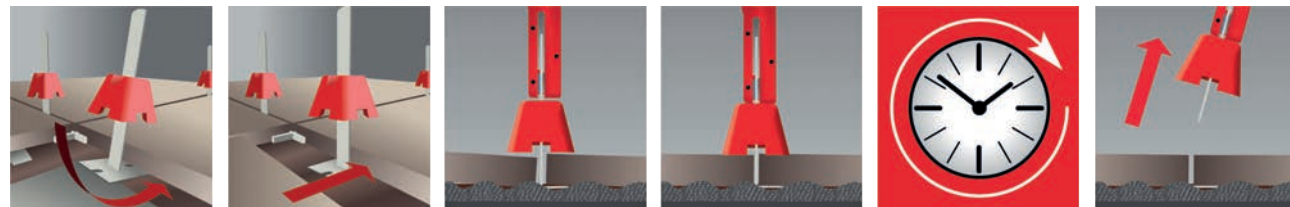
Position strap and cap Lay the tile Attach setting tool Tension until level Wait for glue to dry Remove strap and cap
